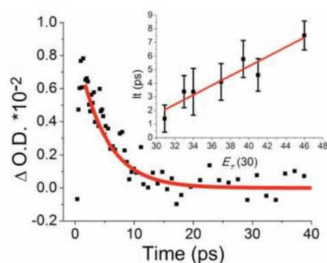
Figure 3. Picosecond decay measured at 600 nm of the OA transient generated by excitation of cyclobutanedione 1 in dichloroethane. Inset: Changes in the lifetime of OA as a function of the solvent polarity parameter E_T(30) .
